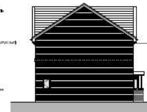
North Elevation @ 1:100
